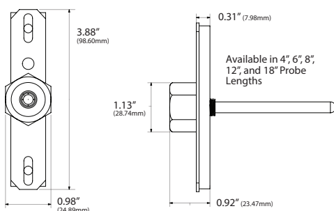
Standard Views
