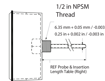
Pictured Above: immersion no well (INW) sensor in Bell Box Enclosure (BB).
