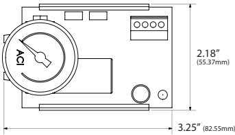
Board with Snap Track
