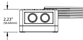
Right View
