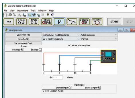
SOIL RESISTIVITY
