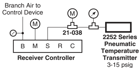
Figure 1 Typical Application.
