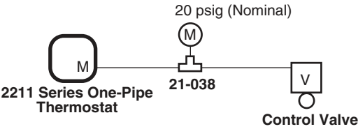
Figure 1 2211 Typical Application.
