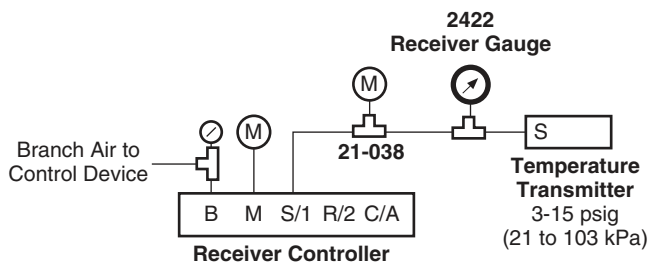
Figure 1 Typical Application.
