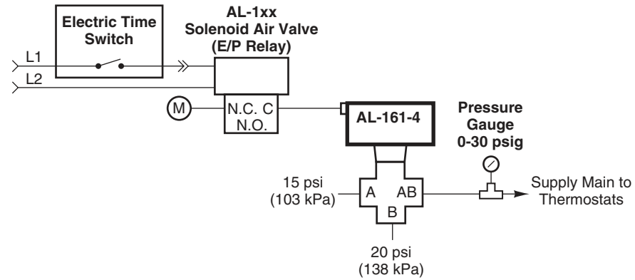
Figure 1 Typical Application.
