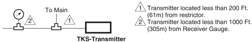
Figure 1 Typical Application.
