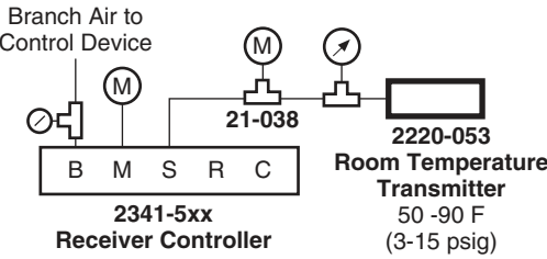
Figure 2 Typical Application.
