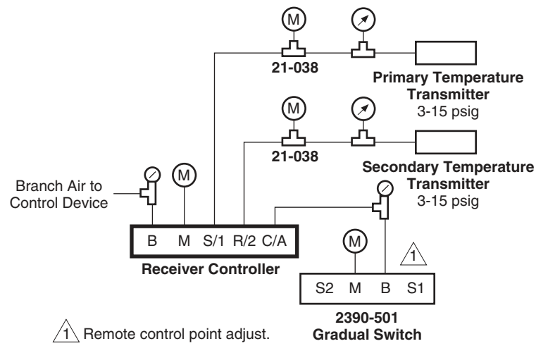
Figure 1 Typical Application.
