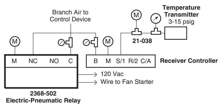
Figure 1 Typical Application.
