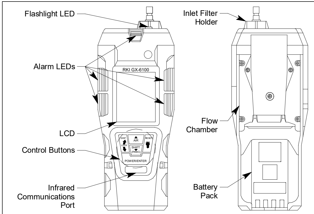
Figure 1: Component Location
