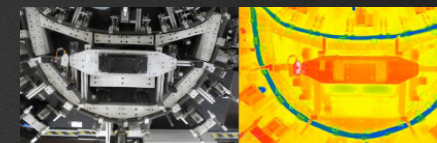
Each green square in this thermal image stands for one of the measurement spots, 19 in this case. The user can define as many measurement spots as needed.
