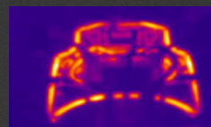
This thermal image shows induction heating at work. The metal parts heat up from room temperature to 100 °C in matter of seconds.
