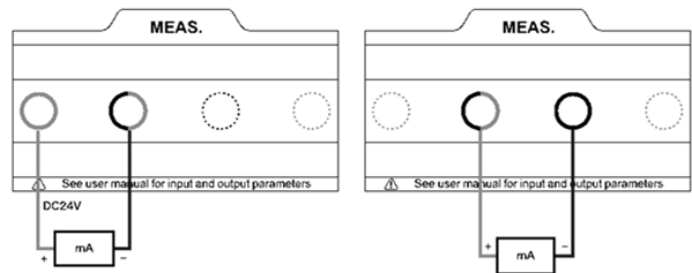
Figure 7 Current Measurement
