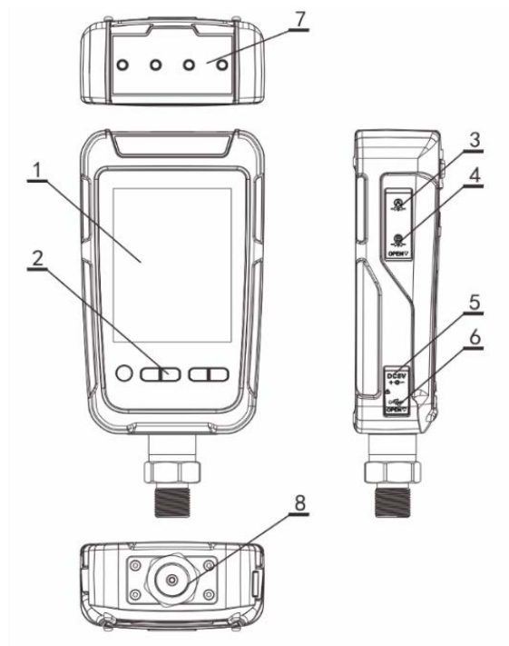
Figure 1 Basic Structure
