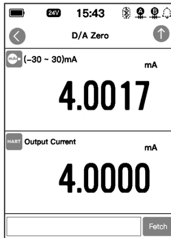
Figure 14 D/A adjustment
