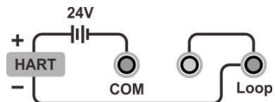
Figure 8 HART-External power and internal resistance
