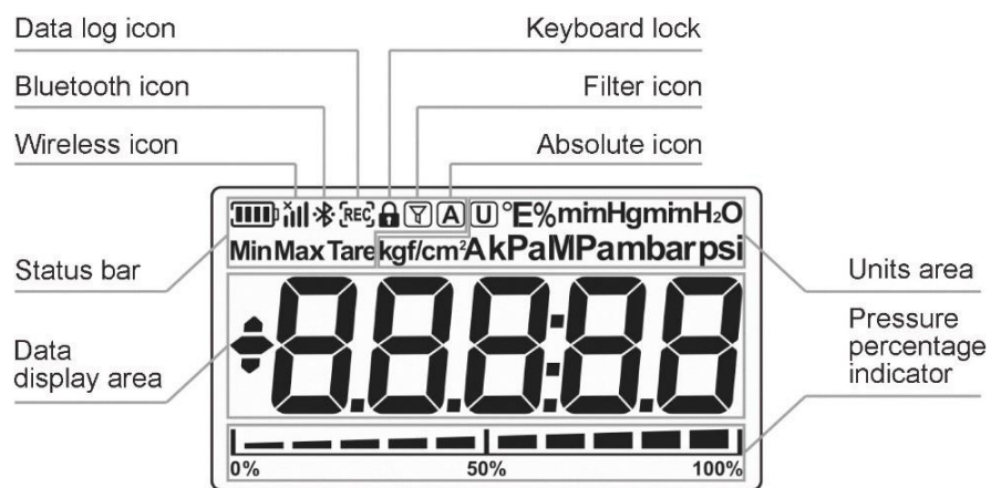
Figure 5 Main Display
