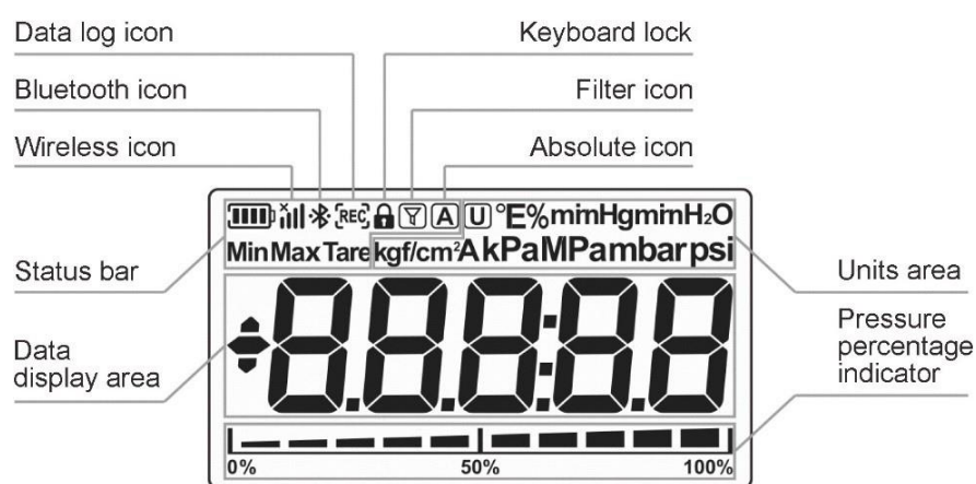
Figure 5 Main Display
