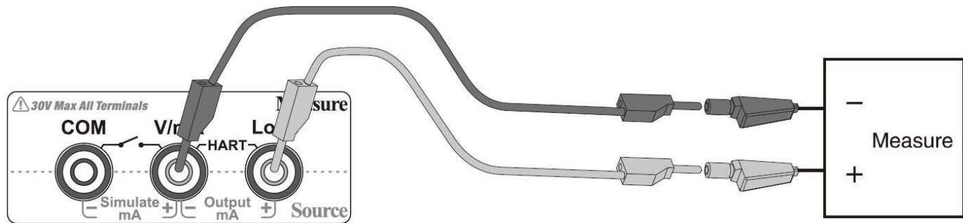
Figure 12 Current Output
