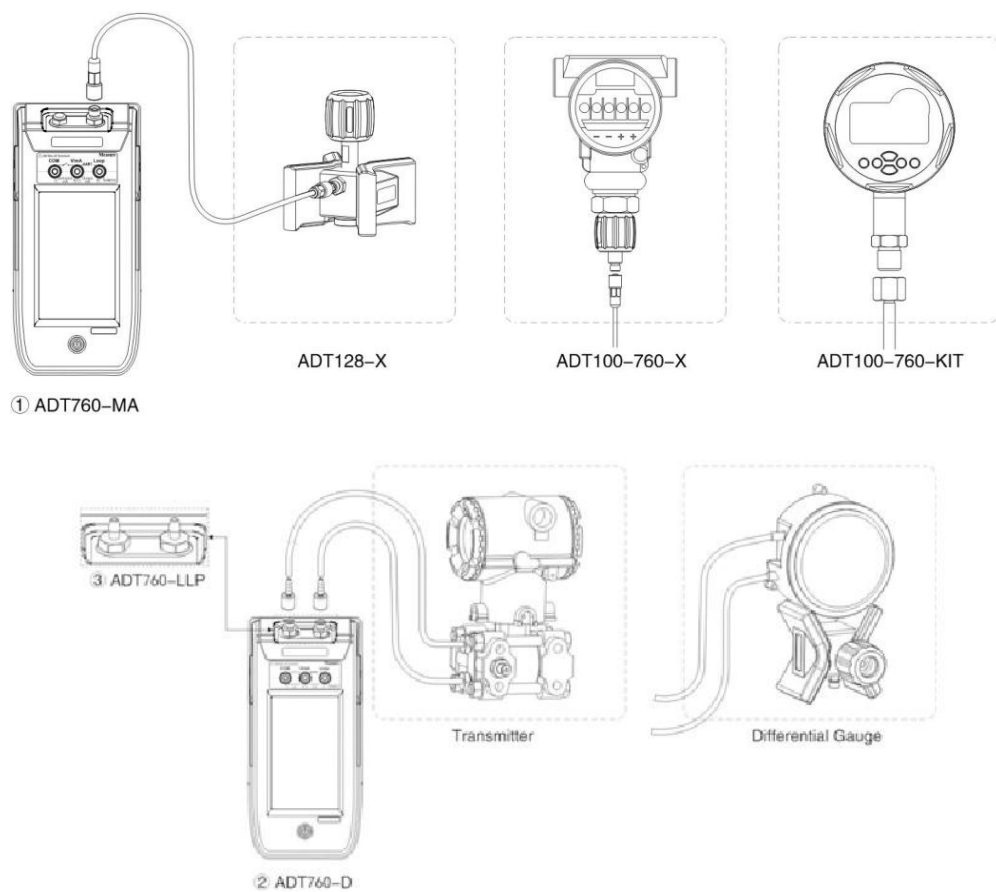
Figure 8 Output Connection
