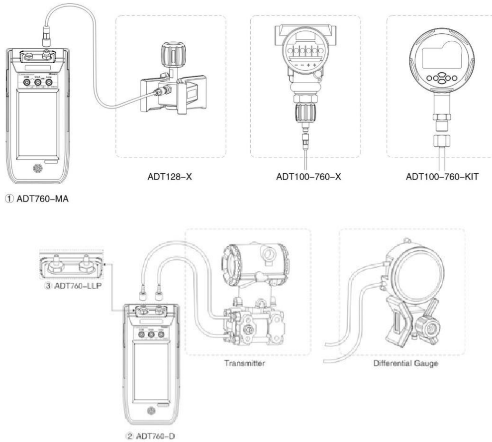
Figure 8 Output Connection
