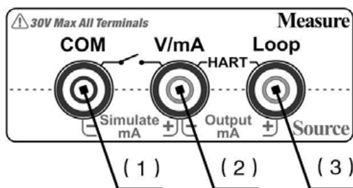
Figure 5 Electric Connection
