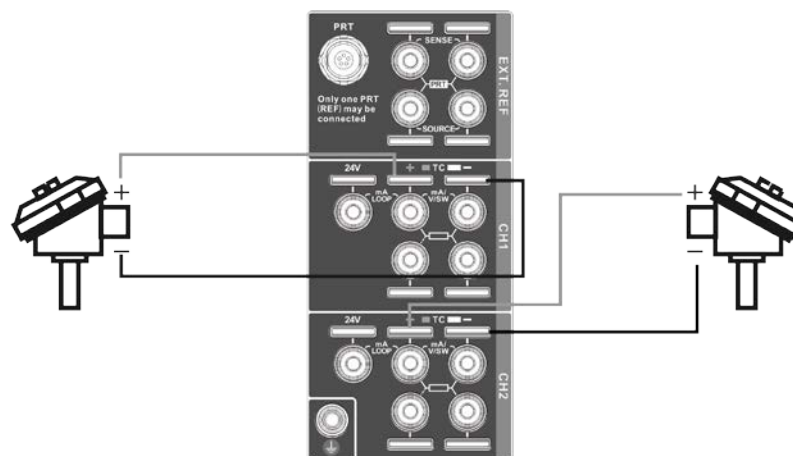
Figure 4 TC Connection
