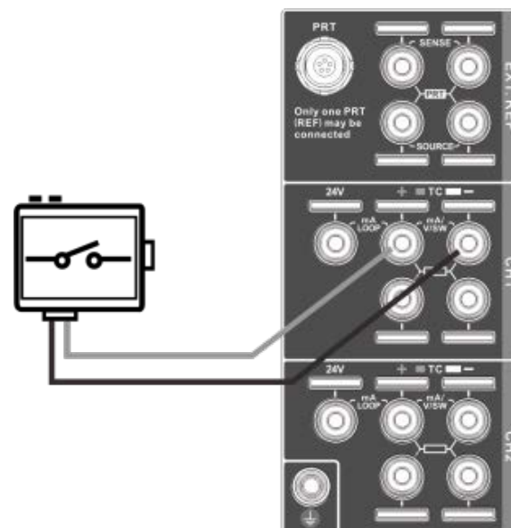
Figure 7 Connection Diagram for Switch Testing
