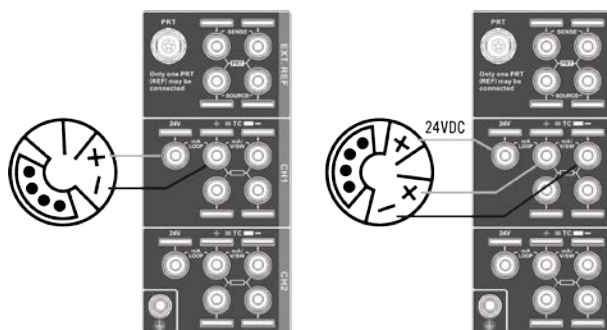
Figure 8 HART Transmitter Connection Diagram
