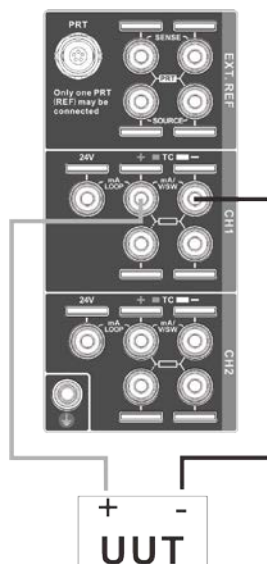
Figure 5 Connection way of Electric Current(mA) Measurement
