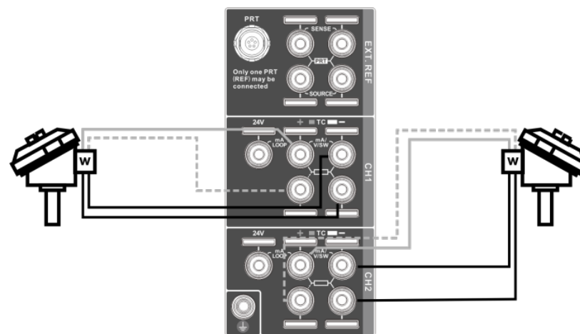
Figure 3 RTD Connection
