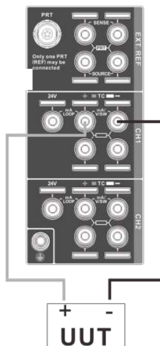
Figure 6 Connection Diagram for Voltage Measurement
