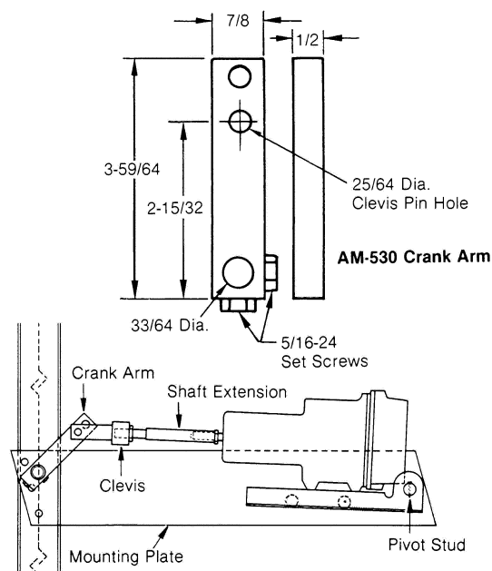
Figure-12 MK-3800 Typical External Pivot Mounted.
