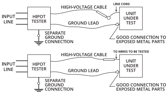
TYPICAL SET-UPS (HIGH-VOLTAGE TEST ONLY)
