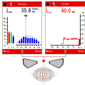
Figure 11 Stop Screens.
