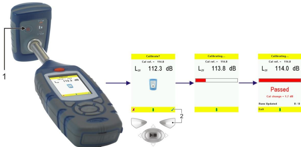
Figure 4. Instrument calibration
