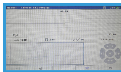
Cable end impedance-matched
