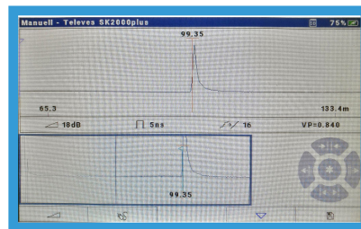
Cable end open-circuited
