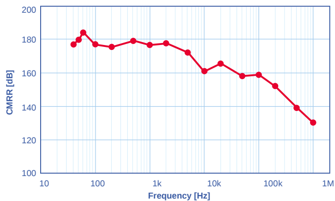
Figure 4. CMRR characteristics
