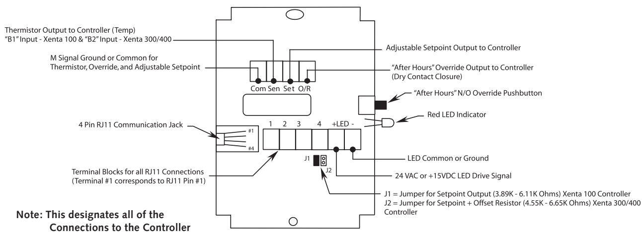
FIGURE 1 - TEMPERATURE SENSOR WIRING DIAGRAM
