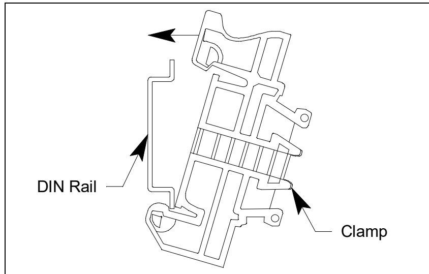
Figure 7: Clamp Installation
