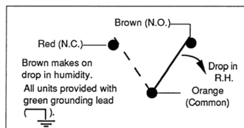
Figure-1 Switch Action and Terminal Identification.
