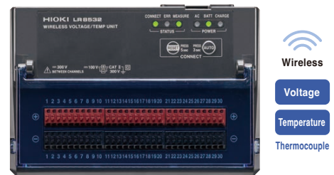
WIRELESS VOLTAGE/TEMP UNIT LR8532
