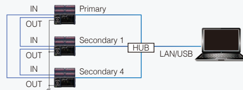
600 CH Analog Synchronous Sampling
