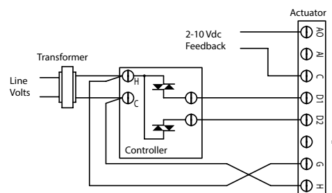
TRIAC SOURCE Application
