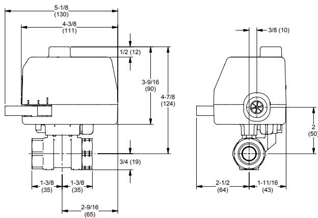
Two-Way Floating/Proportional Non-Spring Return Assembly Shipping Weight: 2.2 lbs (998 g)
