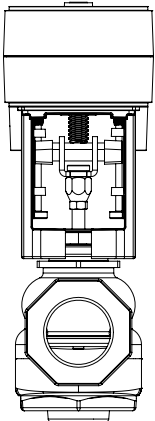
End View
