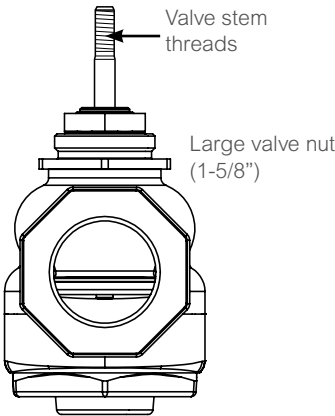
VB-7000 valve body
