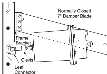
Figure-4 Normally Closed 7" Damper Blade.
