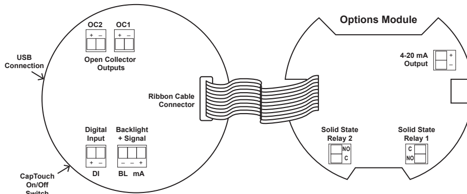
Connections for -L5N Option
