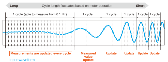
Illustration of auto data update operation
