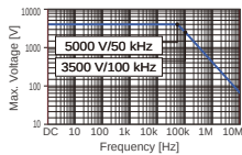
AC/DC HIGH VOLTAGE DIVIDER VT1005
