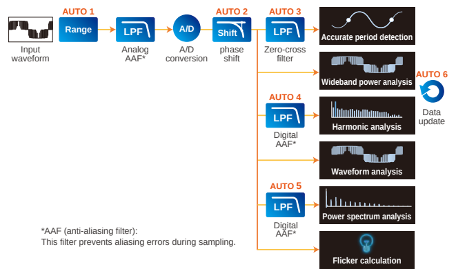
Illustration of auto data update operation
