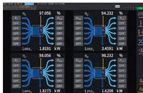
Efficiency and loss calculations (PW8001)
