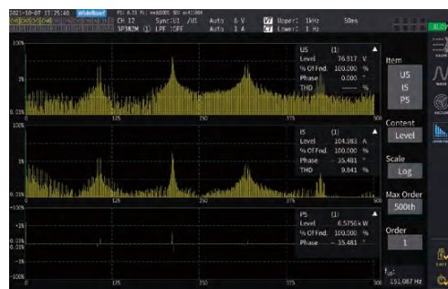
Harmonic analysis of the 500th-order (PW8001)
