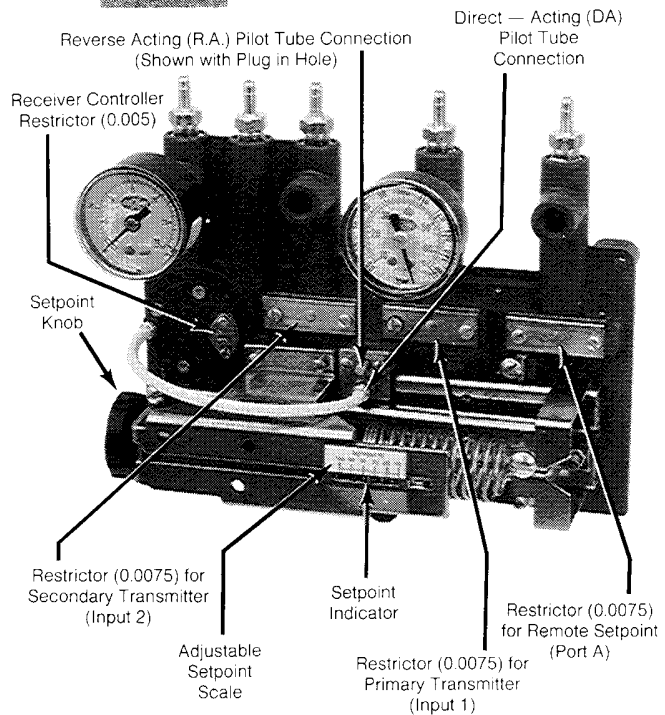
Figure-9 Gasket, Restrictors, Pilot Tube and Setpoint Identification.
