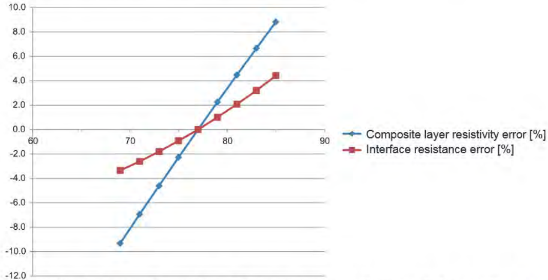
Figure: Effects of incorrectly entering the thickness (representative example for a positive electrode)
