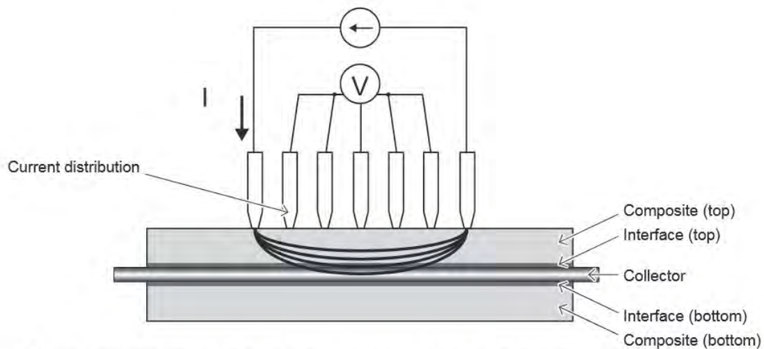
Figure: Cross-sectional diagram of measurement of double-coated electrodes
