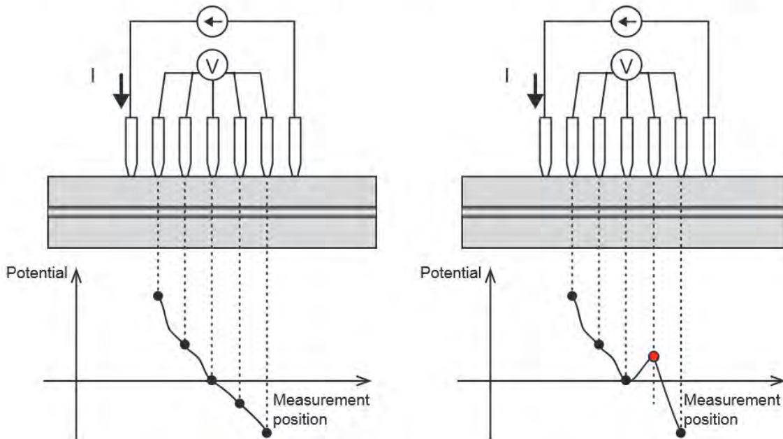
Figure: Illustration of consistency (left: PASS consistency; right: FAIL consistency)
