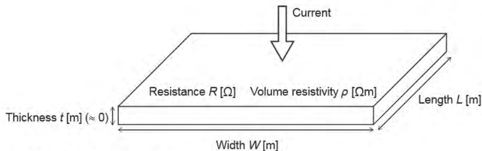
Figure: Definition of surface resistivity
