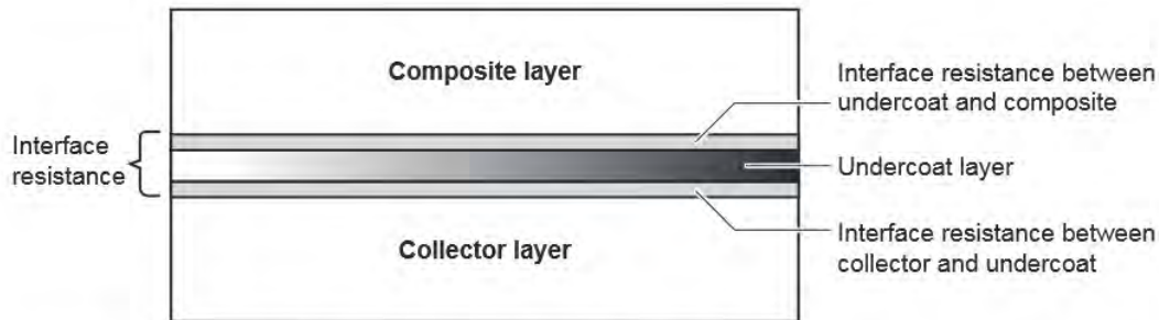
Figure: Diagram showing a cross-section of an electrode using a collector with an undercoat layer
