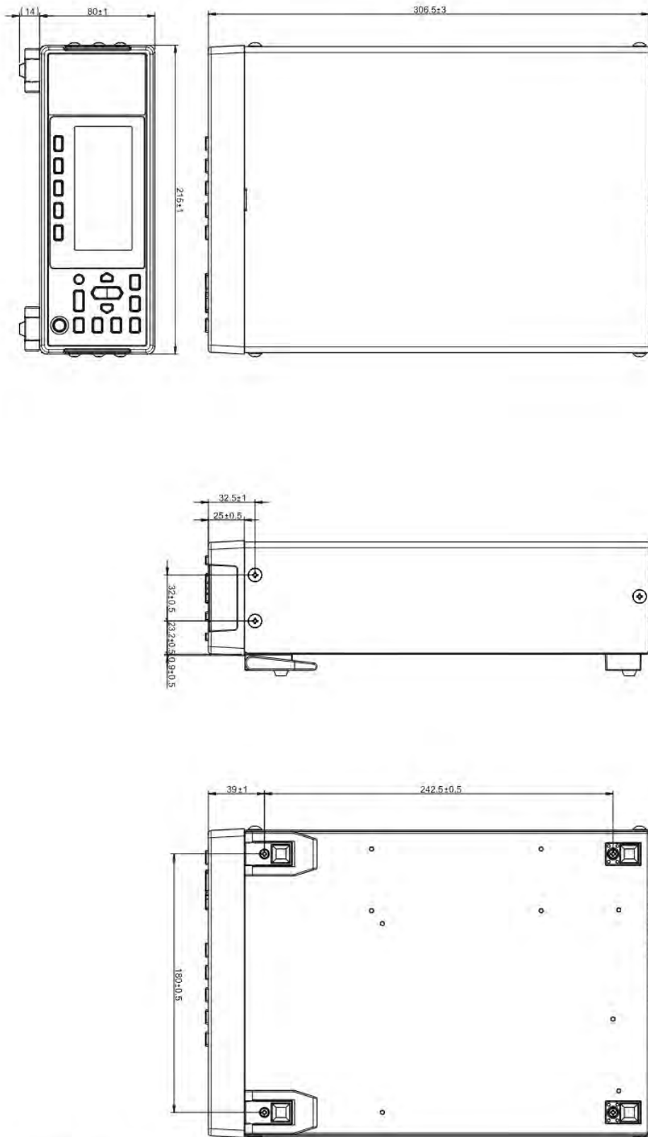
RM2611 Electrode Resistance Meter
