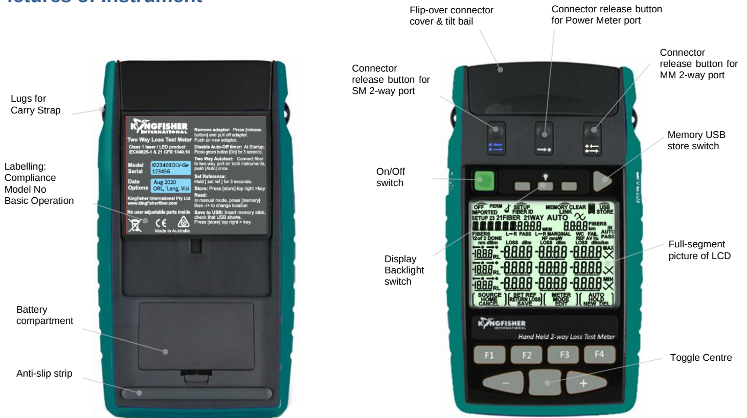
KI23400 / KI27400 HANDHELD 2-WAY LOSS TEST METER
