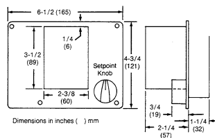
Figure-5 Dimensions of THC-2 and THCR-4.
