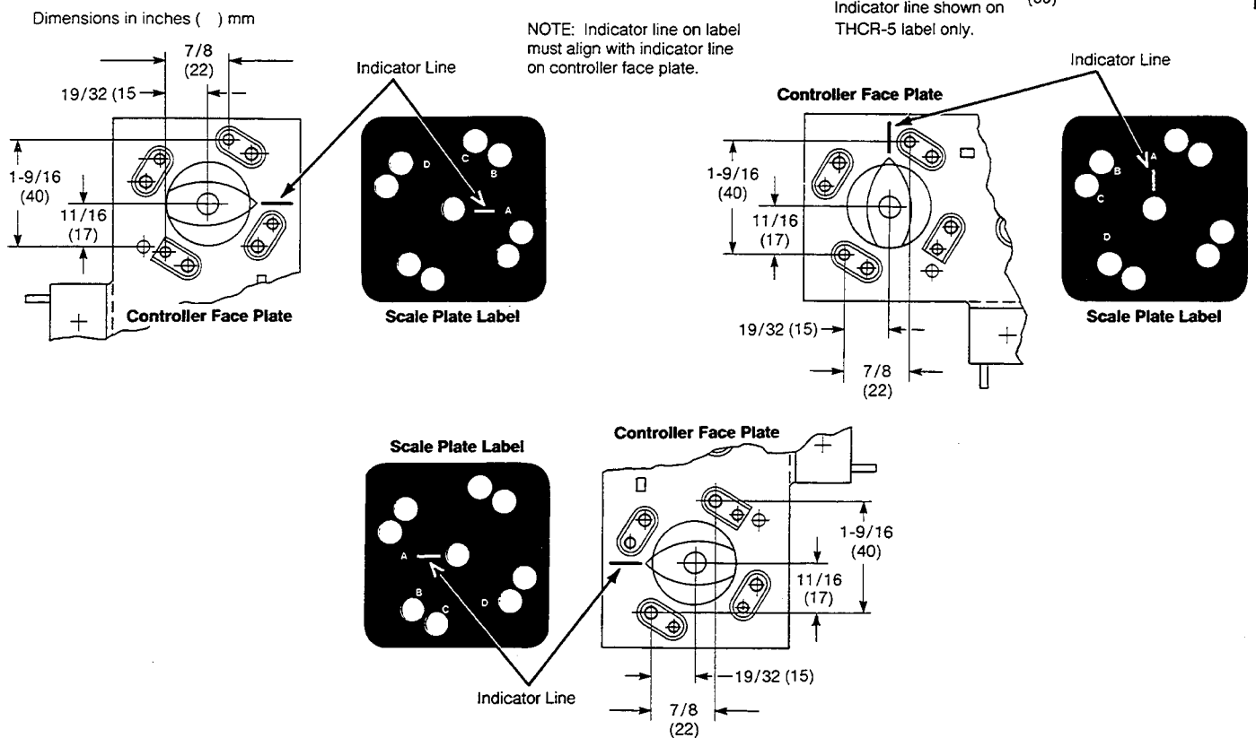
Figure-8 Optional Mounting Dimensions for THCR-5.
