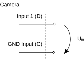
Figure 5-6: Wiring the Digital Input (Example)
