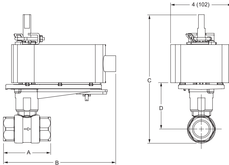
Figure 2. Mx41-6043 or Mx41-6083 with 3-Way Ball Valve.
