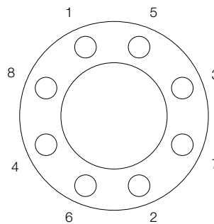
BOLT TIGHTENING SEQUENCE (TYPICAL)
