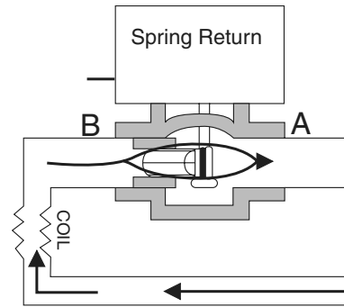
Figure 2 Two-Way Valve Normally Open.
