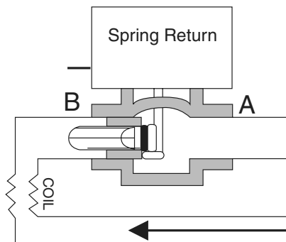
Figure 1 Two-Way Valve Normally Closed.
