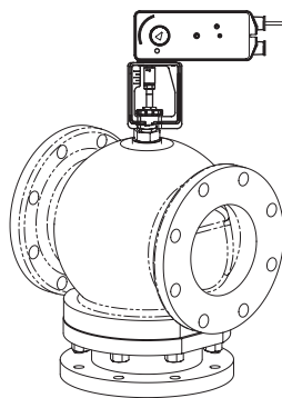
Vx-8303/Vx-9313 with Mx61-720x Direct-Mounted Actuator
