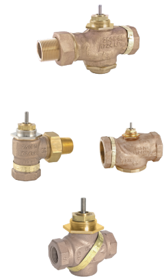
Venta VB-7200 Series 2-way globe valves
