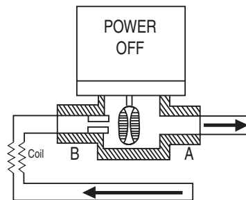
Figure 6 Two-Way Valve with Normally Open Actuator.
