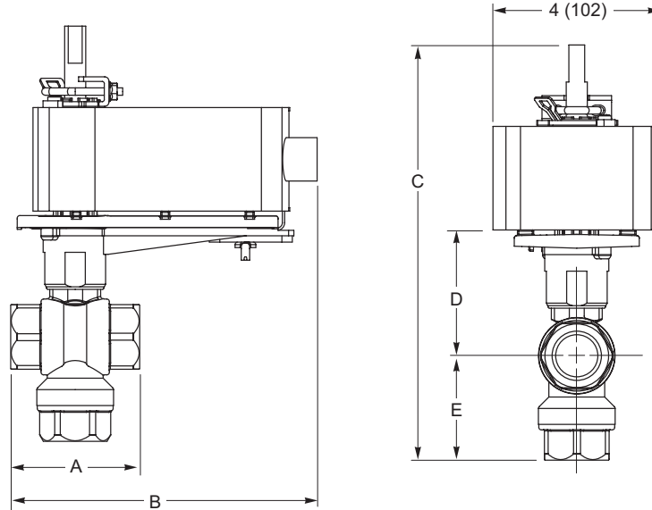
Figure 4. Mx40-704x with 3-Way Ball Valve.
