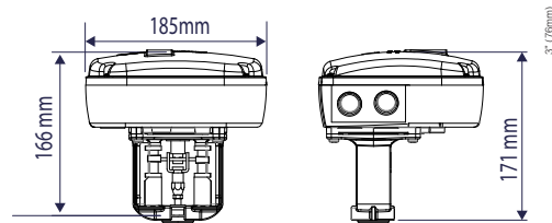
Dimensions for M900AR-VB and M900ARW-VB.
