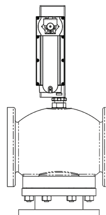
Vx-8303 with Mx41-634x Actuator
