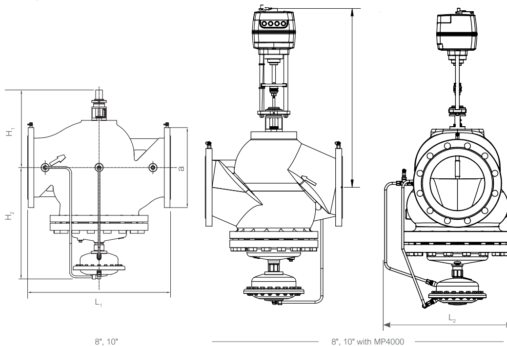
Flanged Valves 8" and 10"
