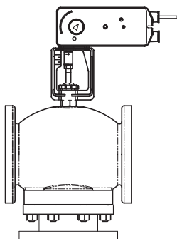
3-Way Linked Globe Valve Assemblies a
