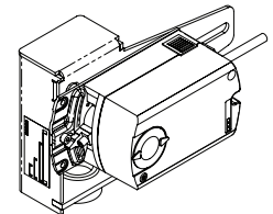
Typical Actuator Mounting
