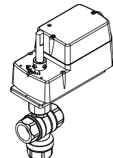
Vx-2313-8xx-9-xx 3-Way Assembly with Mx4D Series Actuator
