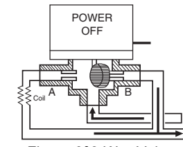
Figure-3f 3-Way Valve in Diverting Configuration Normally Open to the Coil.
